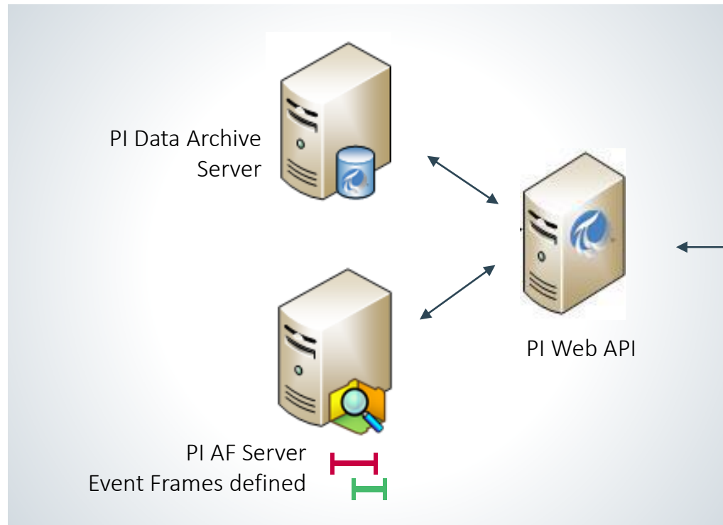
PI System OT Level 3
